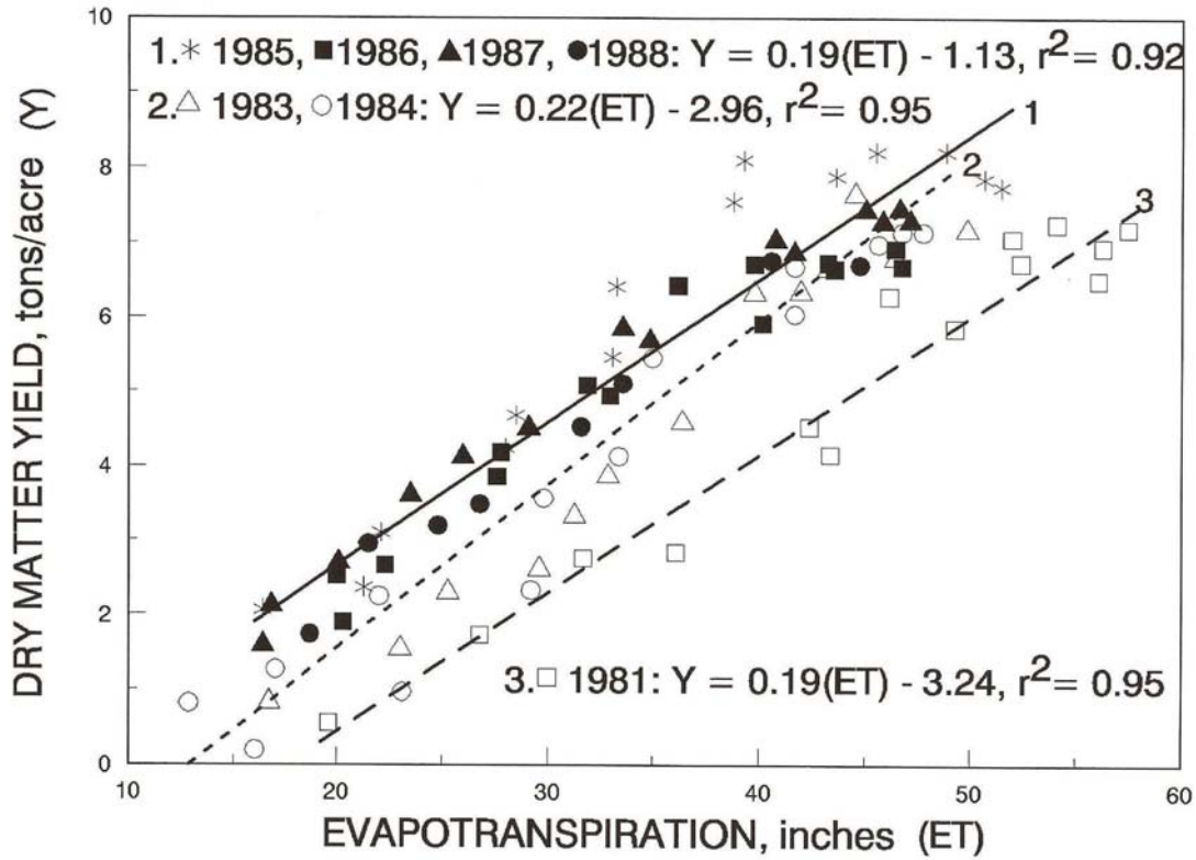
Figure 1. Water use production functions of alfalfa (cv. WL-309) for 7 years of growth at NMSU's Agricultural Science Center – Farmington, NM.
